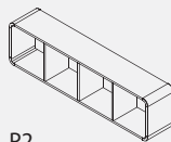
P2 PLAUKTS P/A/Dz - 1480/382/250
